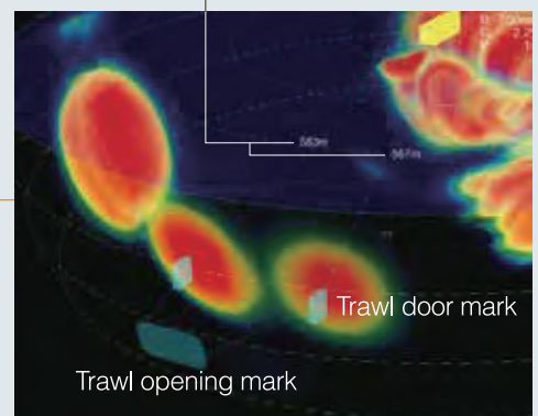
Distance from own ship to the center of the trawl door mark.
